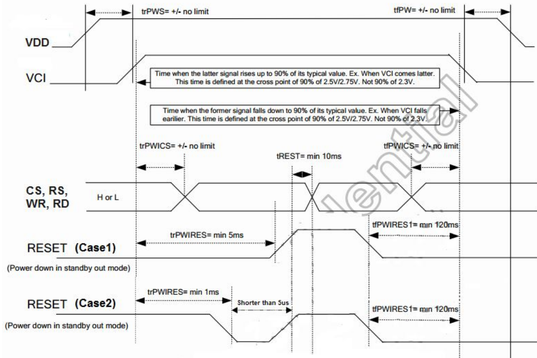
Figure 5.4 Reset Input Timing
