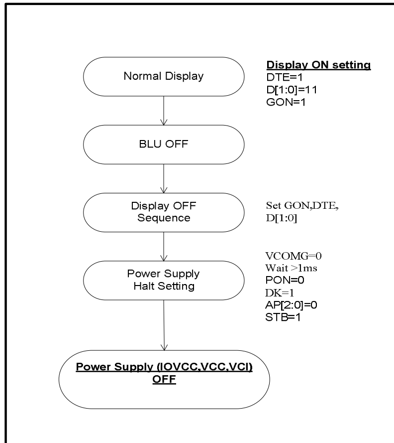
Figure 5.5.1 Power on Sequence
