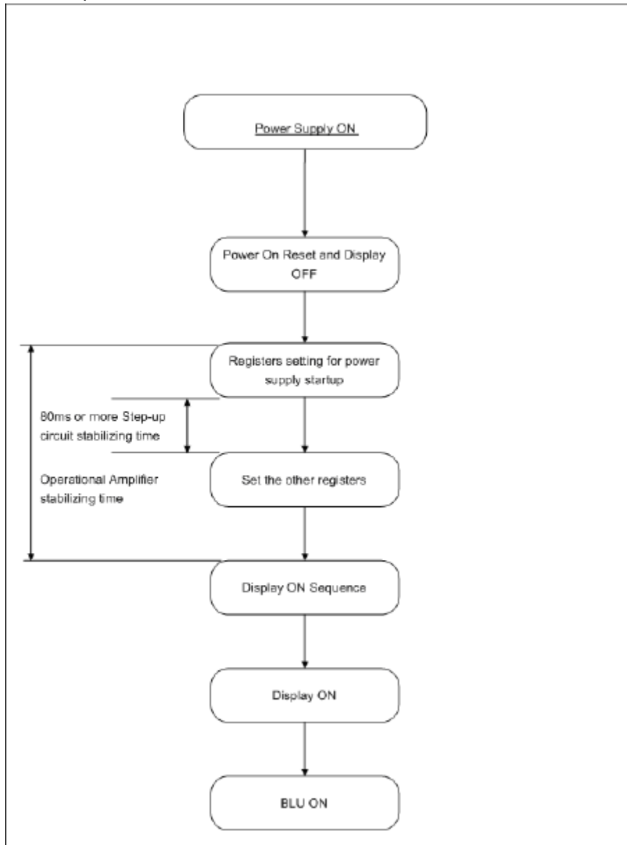
Figure 5.5.1 Power on Sequence
