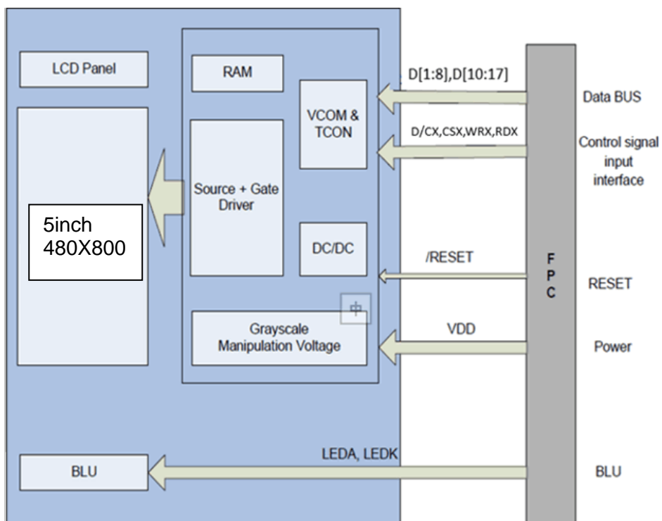
Figure 4.3 LCD module diagram
