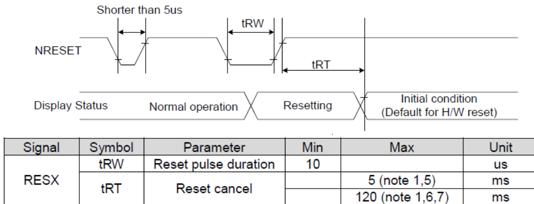
Figure 5.4 Reset Timing Diagram
