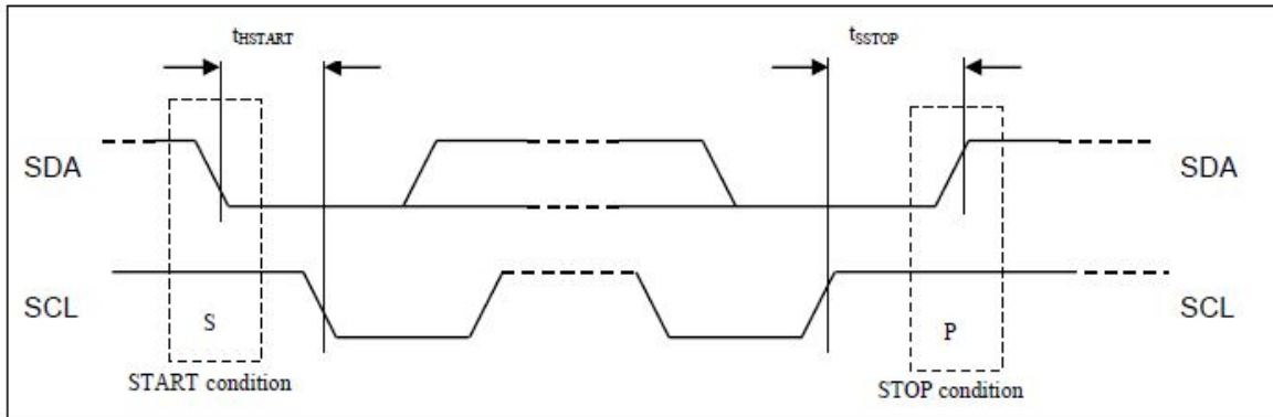
Figure 8-8 : Definition of the Start and Stop Condition
